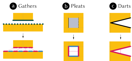
Figure 25: Modeling gathers, pleats, and darts for simulation. Red segments connected by dotted lines are matched and sewn together during simulation. Blue segments are self-matched and fold in half during simulation.
