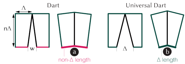
Figure 7: Left: A dart module with width w and height n\Delta = 2\Delta . Right: A universal dart module ( w = \Delta ) ensures that all assembled edge lengths remain integer multiples of \Delta ; edge (b), unlike (a), has length \Delta , and so it may be part of a seam.
